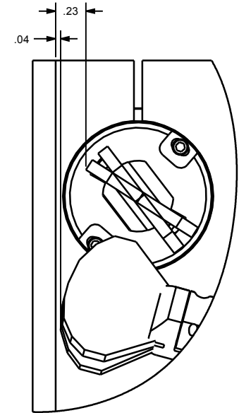
AUXILIARY VIEW SCALE 2:1 DIMENSIONS ON THIS VIEW REPRESENT SMALLEST DISTANCES DURING MIRRORS' FULL ANGULAR RANGE
